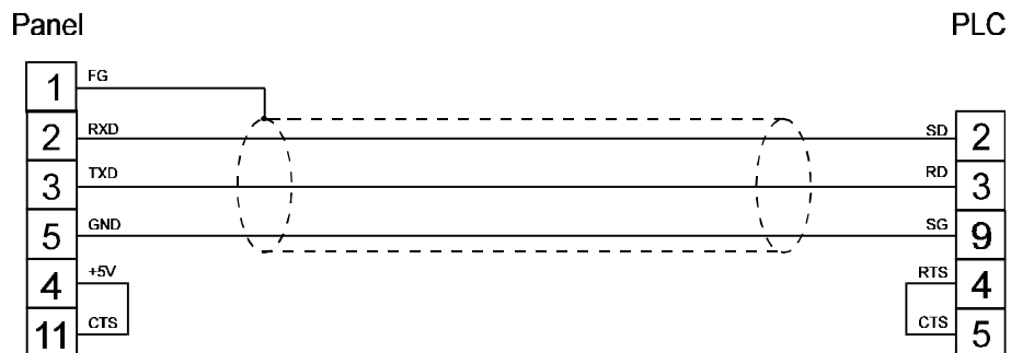
figure 1. Cable diagram
