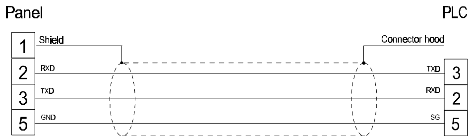
figure 1. Cable diagram
