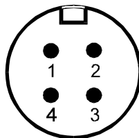
figure 2. Connector end view
