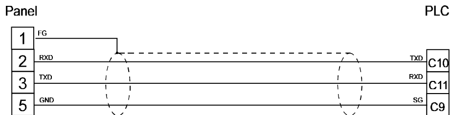
figure 1. Cable diagram
