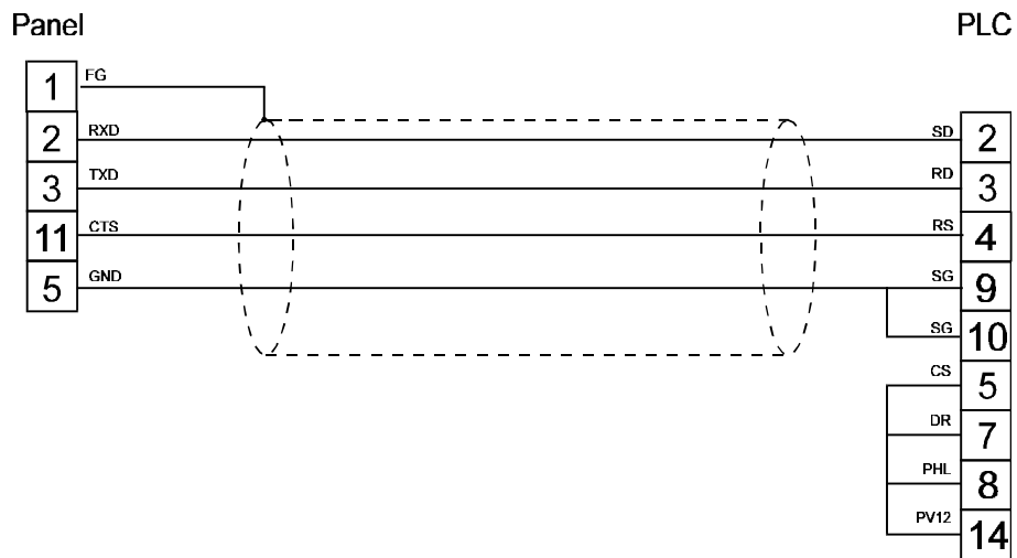
figure 1. Cable diagram
