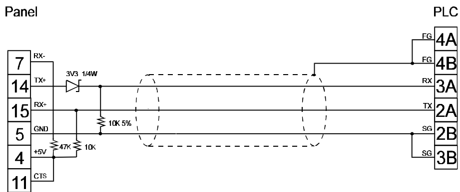
figure 1. Cable diagram
