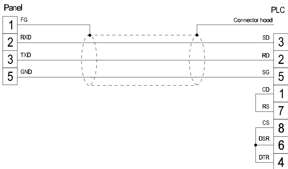
Figure 1. Cable diagram
