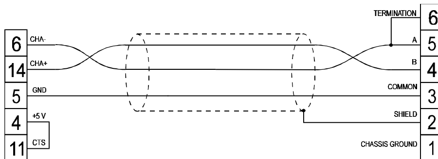
figure 1. Cable diagram
