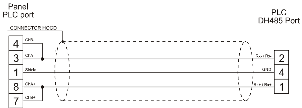
Figure 1. Cable diagram
