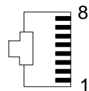
Figure 2. PLC connector (Front view)
