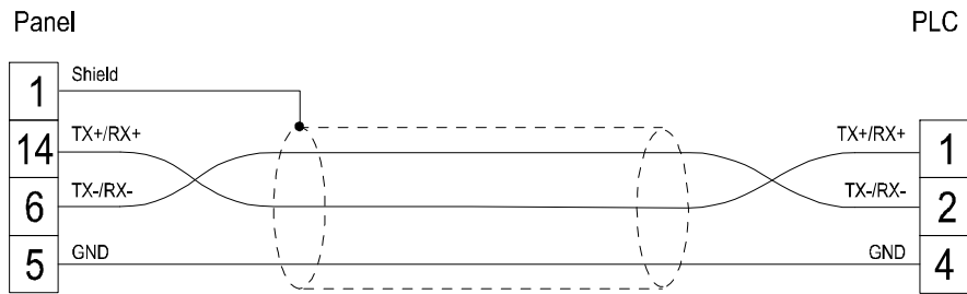
Figure 1. Cable diagram
