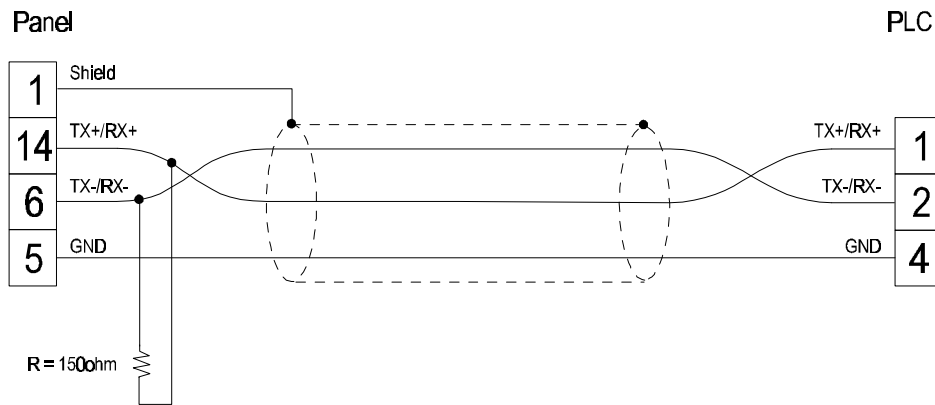
Figure 1. Cable diagram
