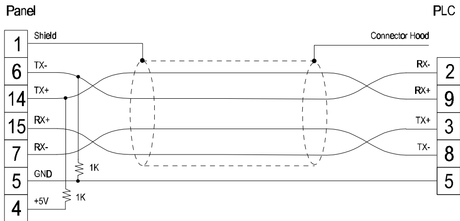
Figure 1. Cable diagram
