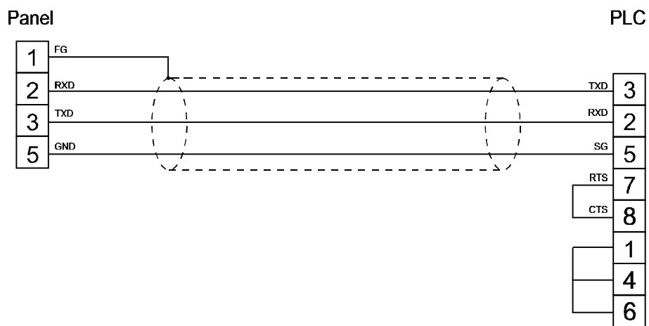
figure 1. Cable diagram
