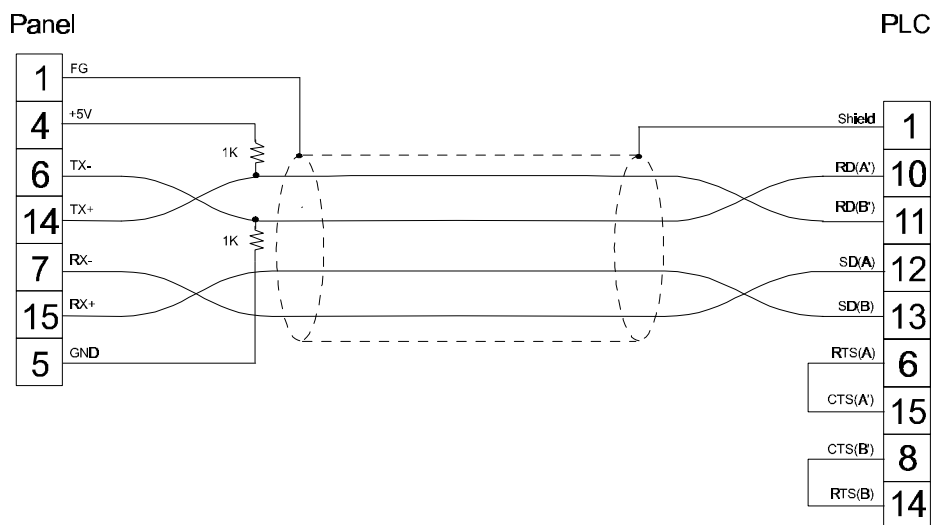
figure 1. Cable diagram
