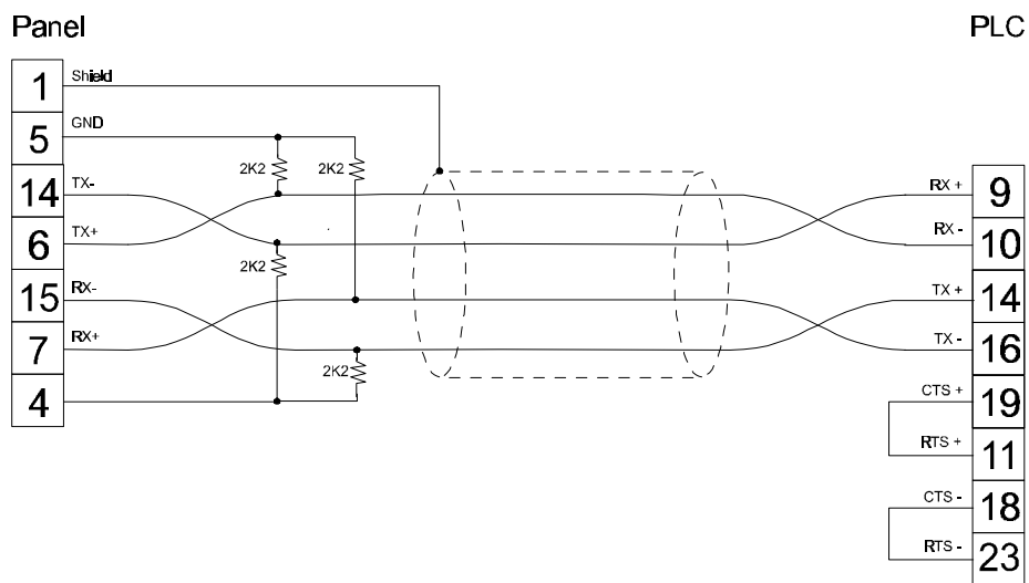
Figure 1. Cable diagram
