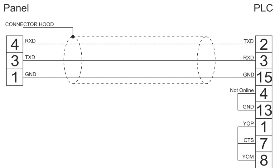
Figure 1. Cable diagram
