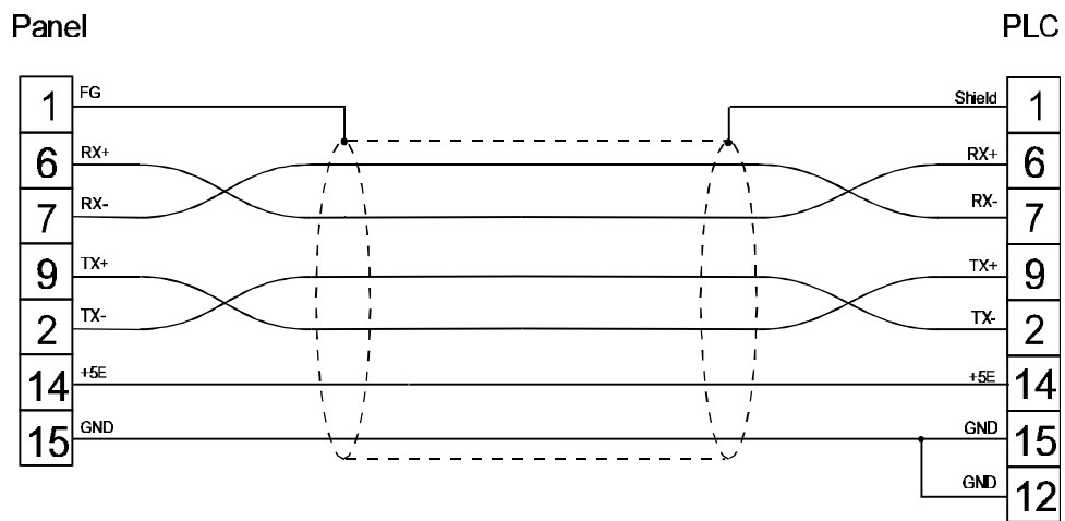
figure 1. Cable diagram
