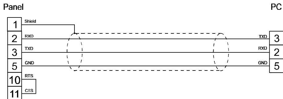
figure 1. Cable diagram
