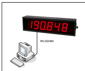
COMMUNICATIONS PC
