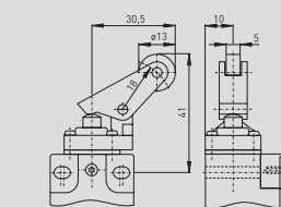
// Parallelhebel WPH Parallel lever WPH
