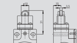
// Parallelhebel WPH Parallel lever WPH
