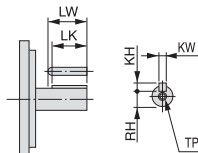
(Key way dimensions)
