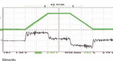
With notch filter
