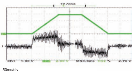
Without notch filter
