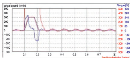
Motor movement
