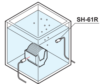
Detecting wafer cassette in quartz tank containing cleaning liquid
