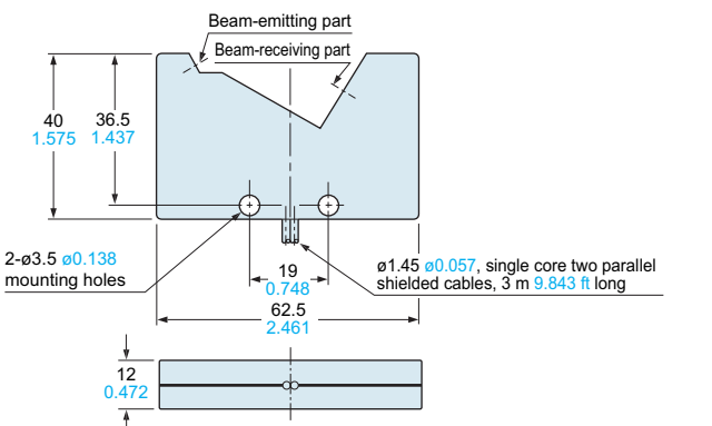
SH-72 Sensor head
