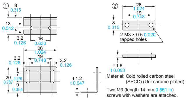
MS-SS3-1 Sensor head mounting bracket (Optional)
