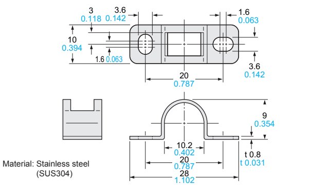
MS-SH6-1 Sensor head mounting bracket (Accessory for SH-61R)
