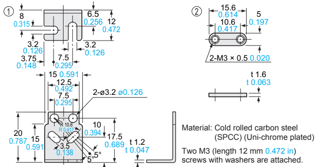
MS-SH6-2 Sensor head mounting bracket (Optional)
