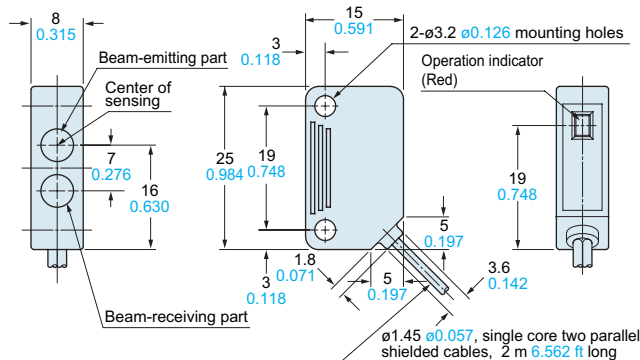
SH-72 Sensor head
