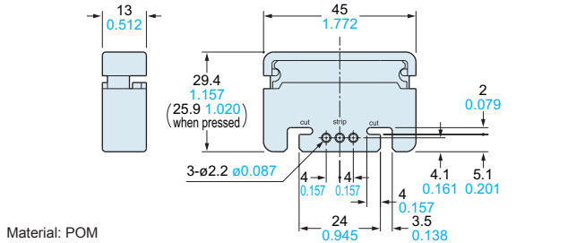
MS-DS-1 Sensor head mounting bracket (Optional)
