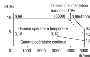
R88M-K1K030H/T (1 kW)
