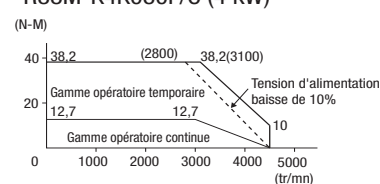
R88M-K4K030F/C (4 kW)
