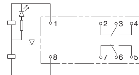
G2R-2-SND, G2R-2-SNDI (c.c.)
