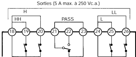
K31-C5 : Relais (5 sorties)
