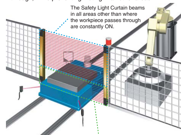
Only the beams of the Safety Light Curtain that would be interrupted by the workpiece are muted.
