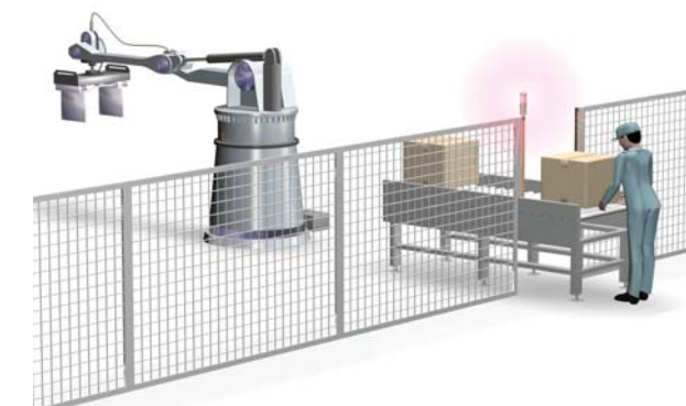
Only the beams of the Safety Light Curtain that would be interrupted by the workpiece are muted.
