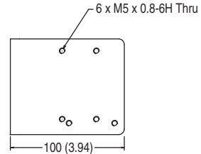
440J-A04N Double Safety Switch Bracket
