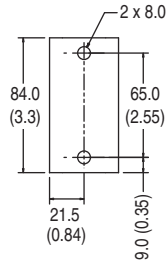
440J-A04N Double Safety Switch Bracket
