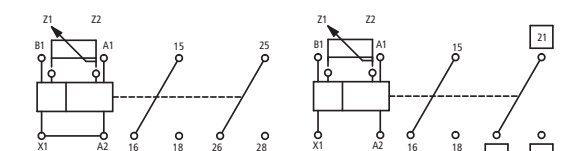
12 OFF-DELAY 16 ON- and OFF-DELAY 22 FLEETING CONTACT ON DE-ENERGIZATION 82 PULSE SHAPING CONTACT
