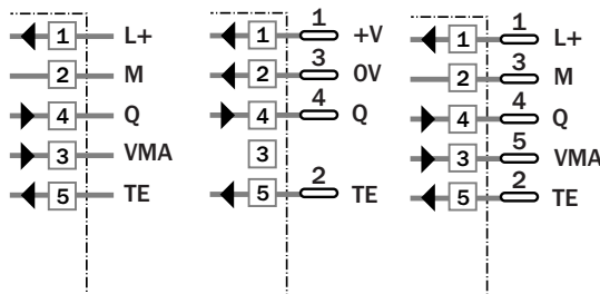
Bornier 4 pôles, M 12 5 pôles, M 12
