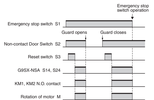
Timing chart
