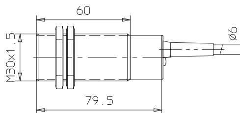
E2EL-X15M□-L 2M
