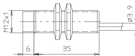
E2EL-X4M□ 2M
